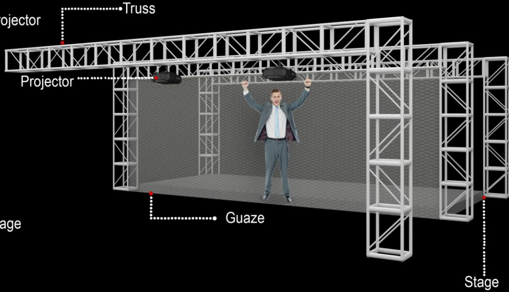
Front Projection
